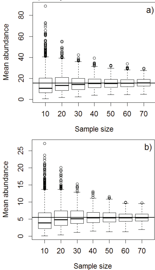
Fig. 1. Distribution of mean abundance obtained from empirical parasite data sets by BLB for different sample sizes for Ligophorus cephalii (a) and L. mediterraneus (b). The box spans the first and third quartiles; the median is marked inside the box by thick horizontal line; minimum and maximum values excluding outliers (whiskers) and outliers (circles); the straight line is the empirical mean abundance.
